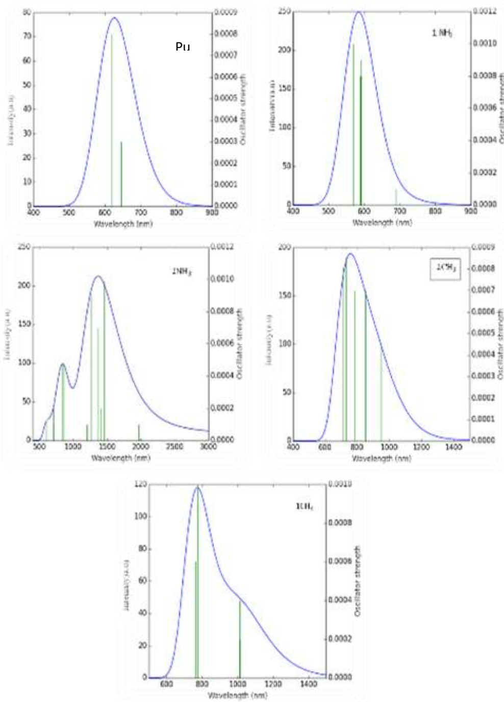
Figure 3: UV-Vis Spectra of the compounds.
