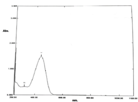
Figure(2): UV-Vis Spectrum for the (PAC) ligand
