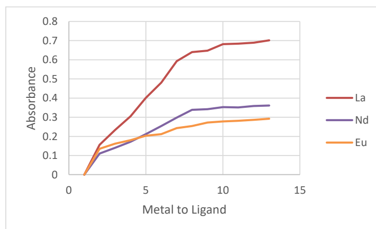
Figure(1) : Mole Ratio Plot For The PAC. Complexes Solutions At \lambda_{max} .
