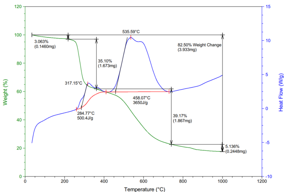
Figure(9):Thermogram for the [(PAC)]ligand
