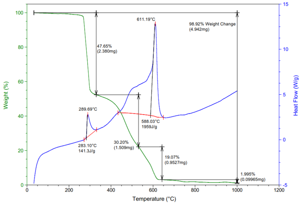
Figure(10): Thermogram for the [Nd(PAC)_2]Cl complex
