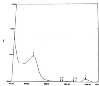
Figure(5):UV-Vis Spectrum for the [Nd(PAC)2]Cl complex
