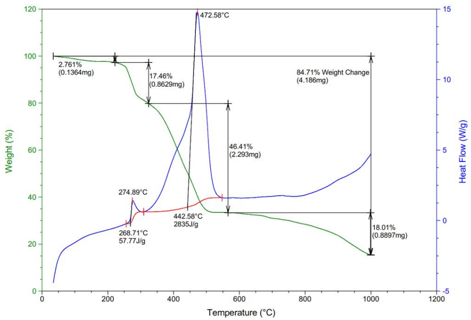
Figure(11): Thermogram for the [La(PAC)_2]Cl complex
