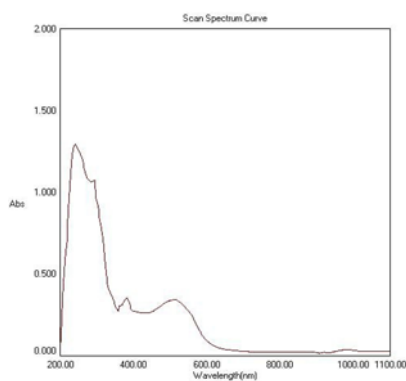
Figure (4):UV-Vis Spectrum for the [La(PAC)2]Cl complex
