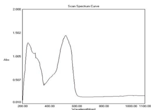
Figure (3):UV-Vis Spectrum for the [Eu(PAC)2]Cl complex
