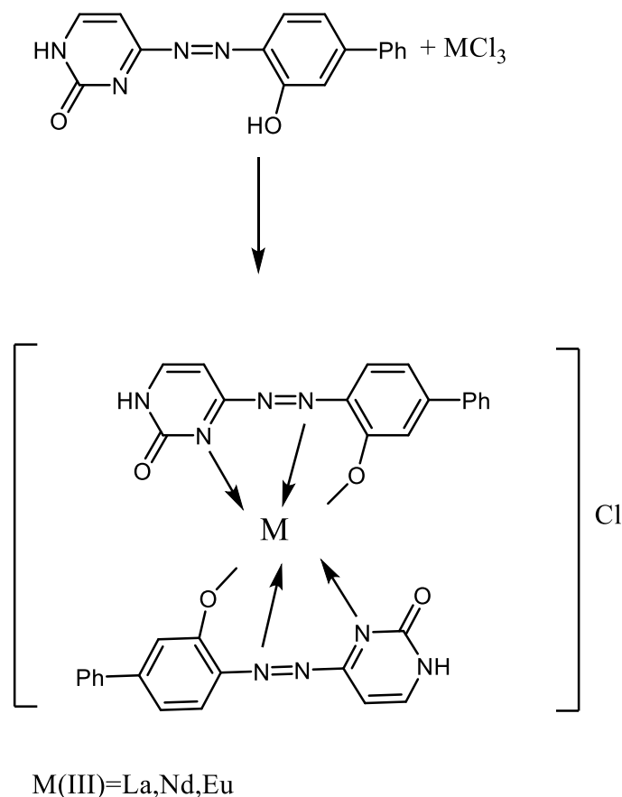
Scheme(2): Synthesis of complexes
