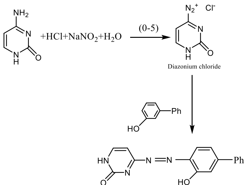
Scheme (1): Synthesis of ligand (PAC)
