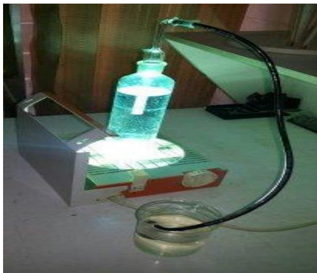
Figure 2, The electrolysis cell
