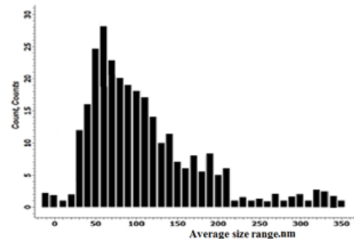
Figure 4b , granularity normal distribution of . nano photocatalysts (SnO 2 -ZnO)
