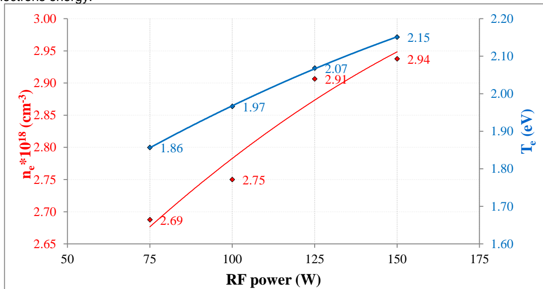
Figure 6. Variation of T_e and n_e with the rf power.
