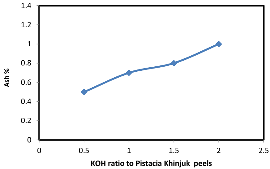
"FIGURE 3",The relationship between the added (KOH) ratio With Ash content in activated carbon
