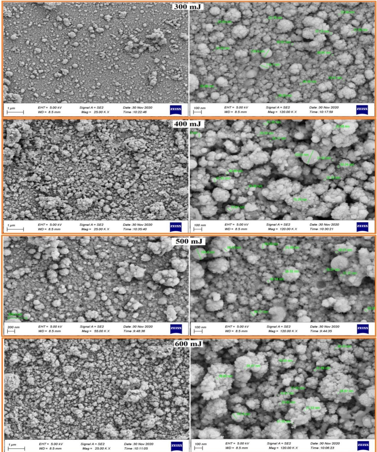
Figure (2): FESEM images at two magnification powers for CdO:NiO composite thin films Which are prepared by different laser energies.
