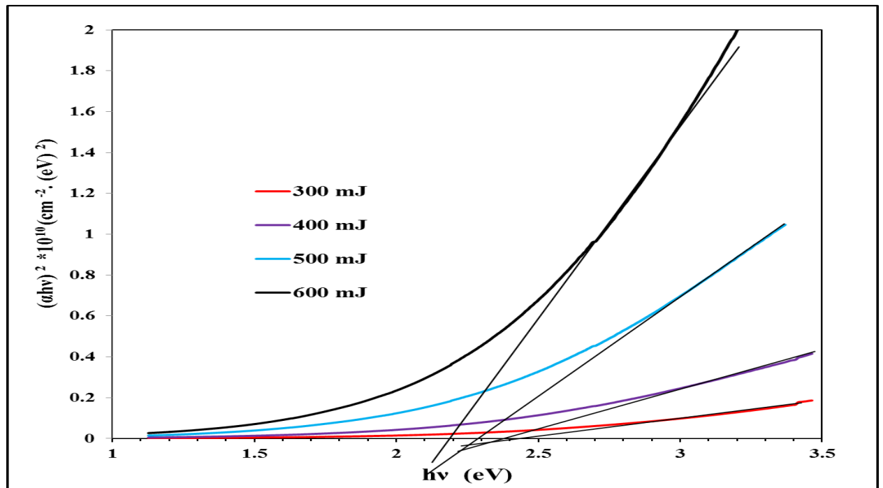
Figure (5): Energy gap for CdO:NiO thin films are prepared by different laser energies.
