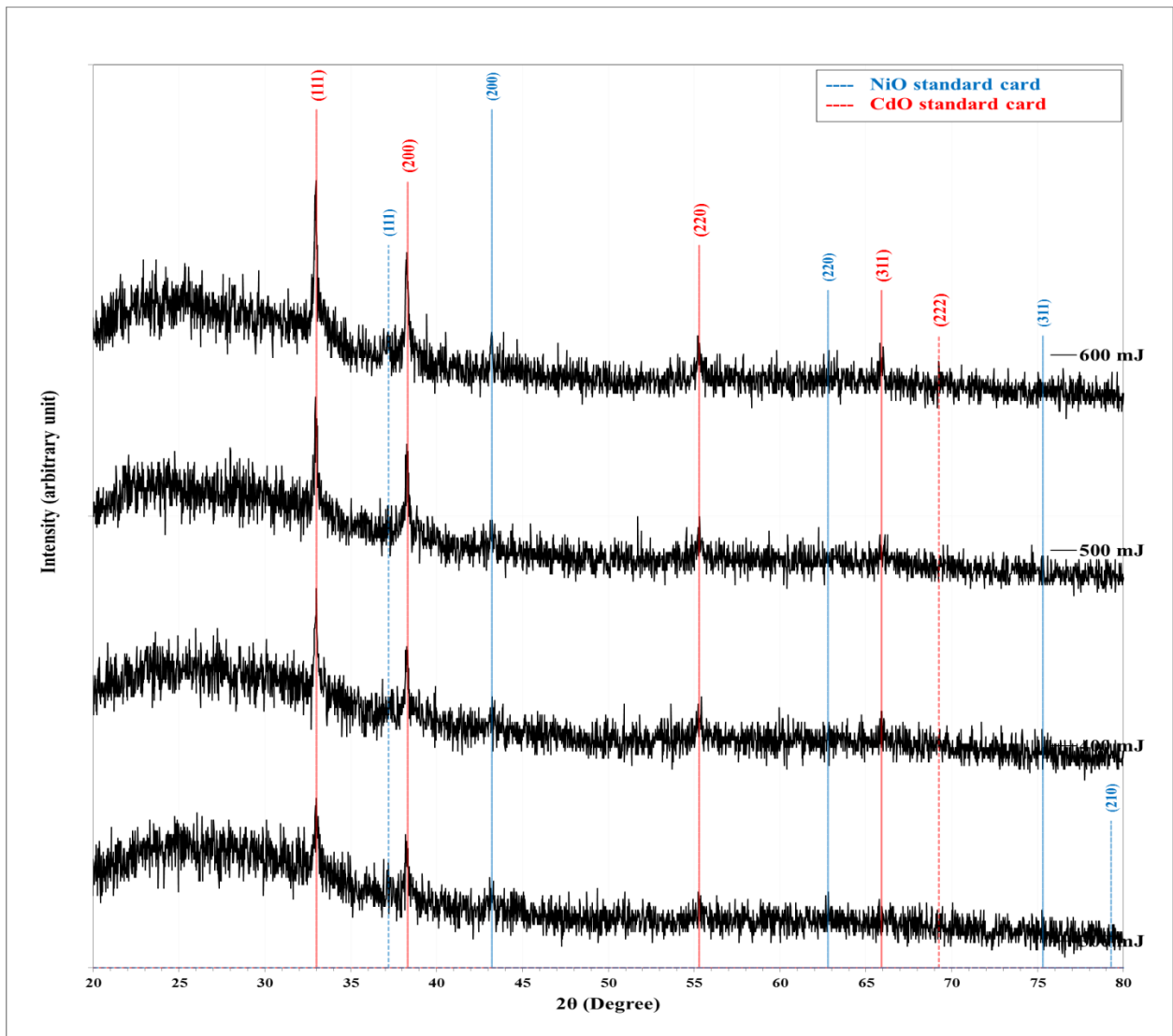
Figure (1) X-ray diffraction patterns for CdO:NiO composite thin films prepared by different laser energies.
