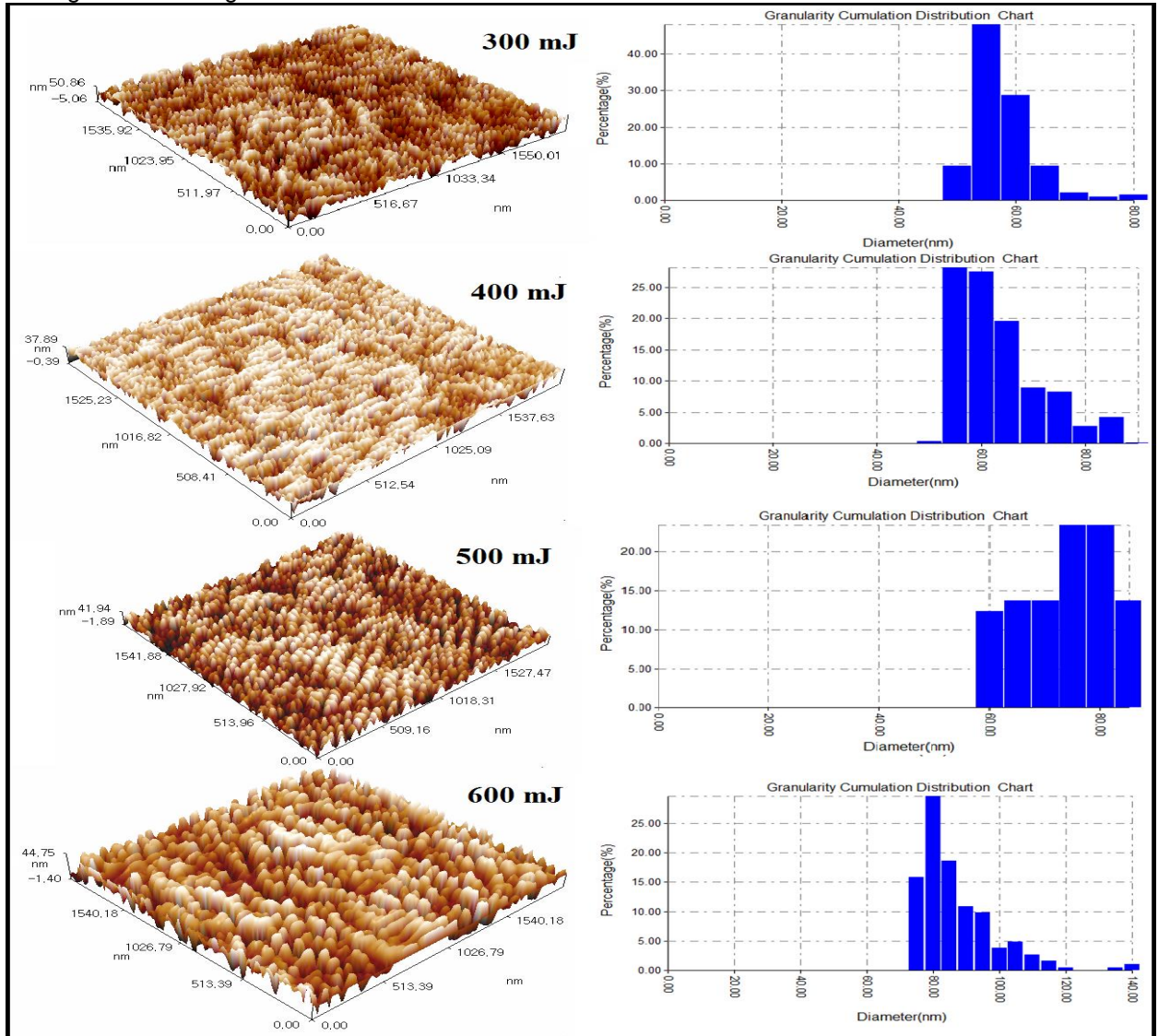
Figure (3): AFM images for CdO-NiO thin films and their granulometry cumulating distribution.
