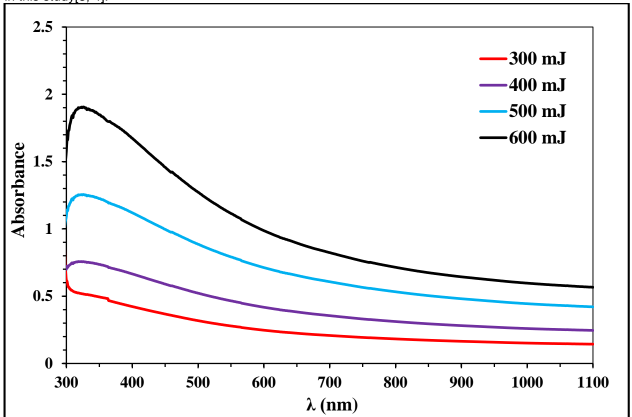
Figure (4): UV-visible absorbance spectra for CdO:NiO thin films are prepared by different laser energies.
