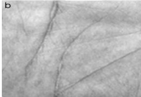
Figure 6: ROI Extraction [10]
