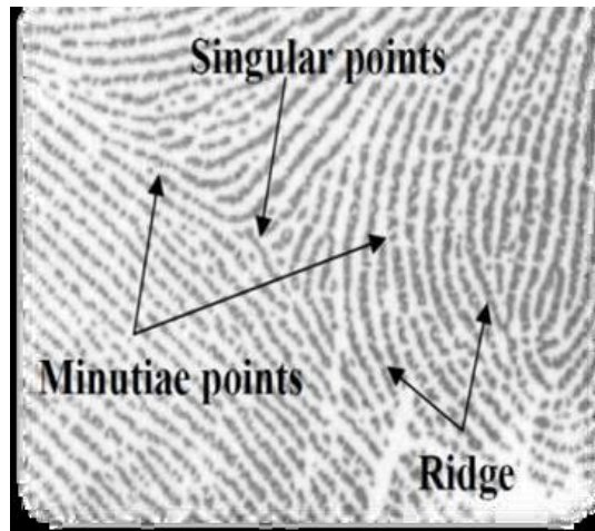
Figure 1: Palmprint Features [9]
