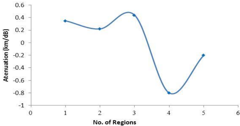
Figure (14): The attenuation(dBm/Km) versus with Number of regions of FBG.
