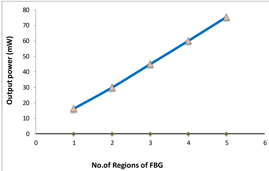
Figure (11): The output power (mW) versus Number of regions of FBG.
