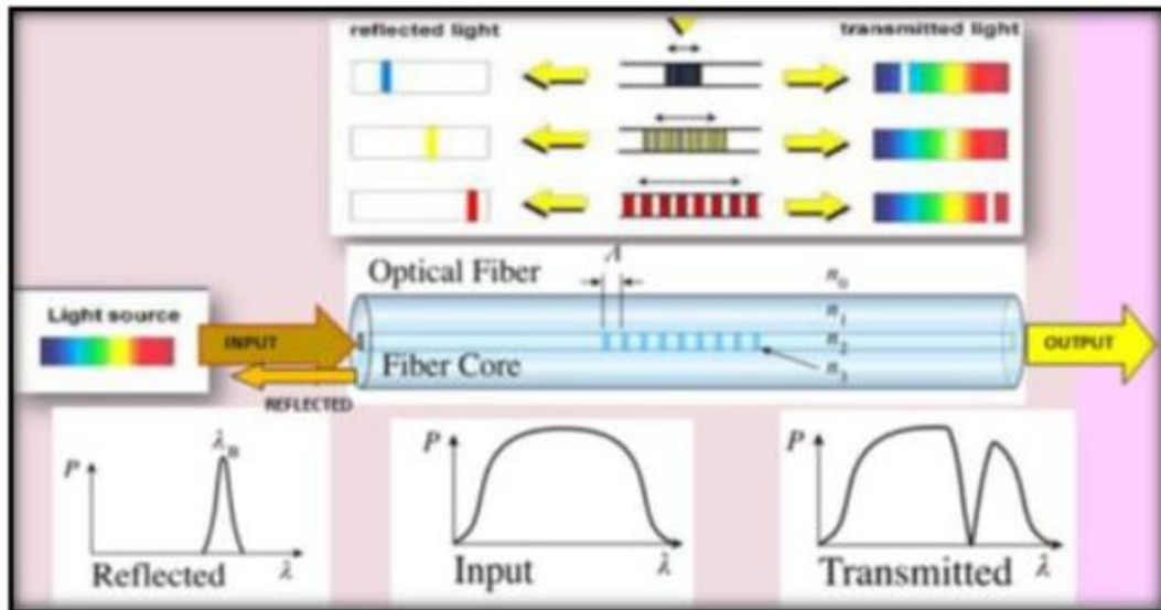
Figure(2): The principle of Bragg's light [8]. Table (1): List of Abbreviations
