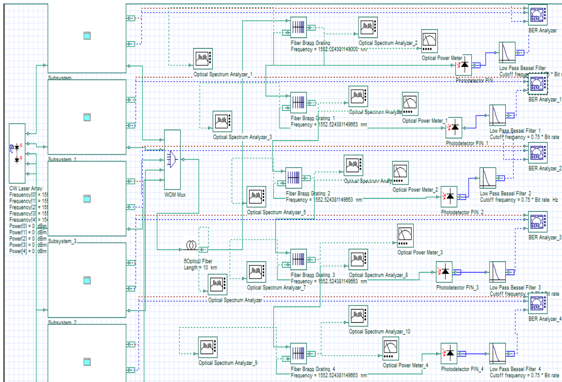
Figure (7): The designed model of simulated system in five regions FBG with Optisystem software.
