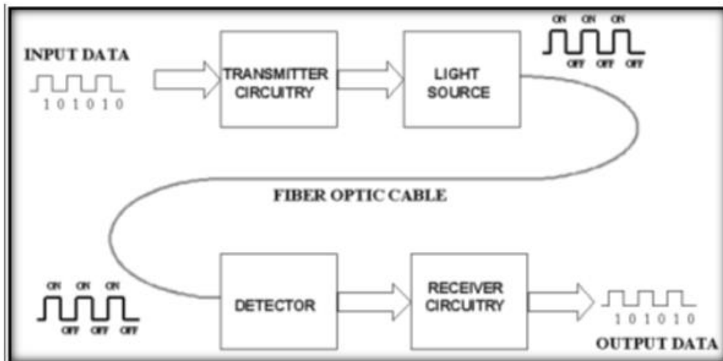
Figure(1): Basic system of fiber optic communication [3].
