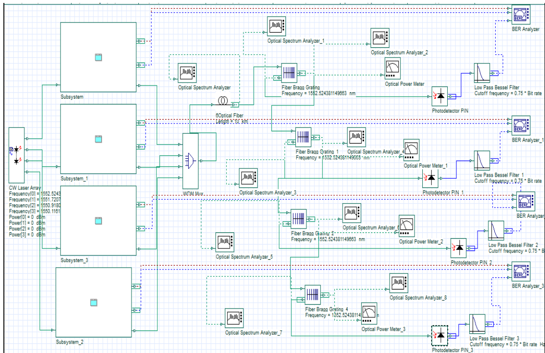
Figure (6): The designed model of simulated system in four regions FBG with Optisystem software.
