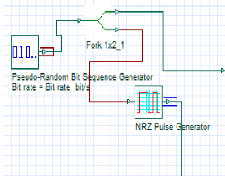
Figure (8): The electrical signal source
