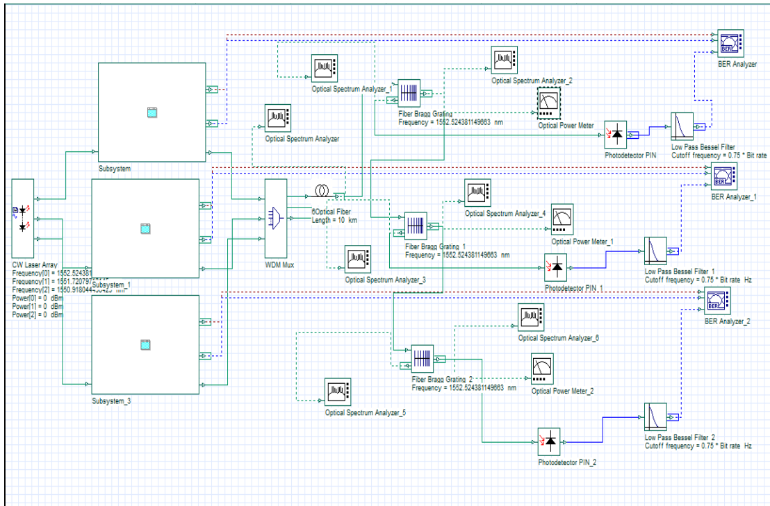
Figure (5): The designed model of simulated system in three regions FBG with Optisystem software.
