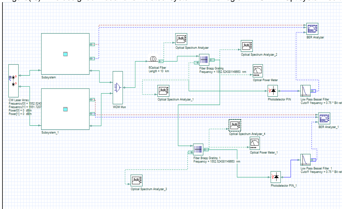
Figure( 4):. The designed model of simulated system in two regions FBG with Optisystem software.
