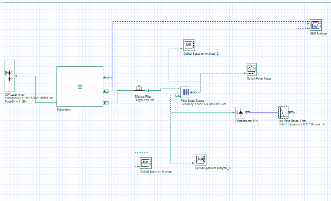
Figure (3): The designed model of simulated system in one region FBG with Optisystem software.
