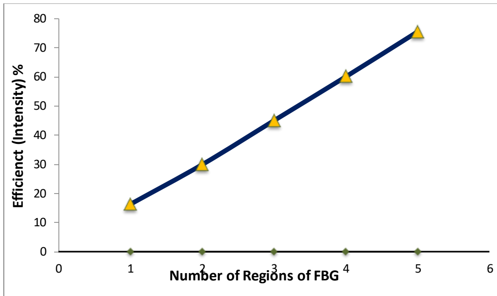
Figure(13): The Efficiency(Intensity%) figure versus Number of regions of FBG.
