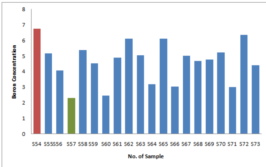
Figure (3): concentrations of boron in water samples in parts of the marine environment in Iraq using (SSNTDs)
