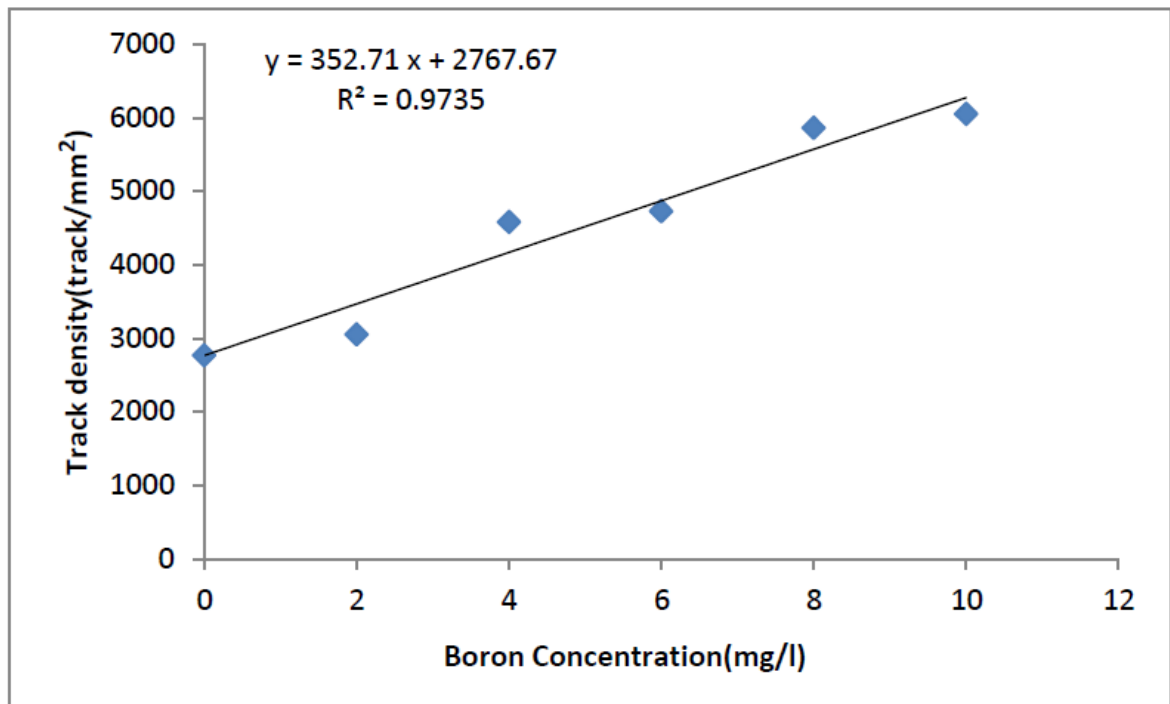
Figure (2) shows the relation between the concentration of boron and track density
