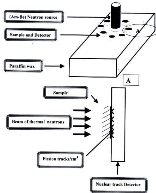
Figure (1) Shows the sample and irradiation of detector in front of neutrons source
