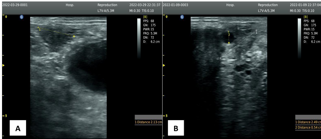
Figure 1. A, An ultrasound image of the ovary in postpartum anestrous cows shows gray iso echoic with a high echoic border and absence of follicles by using a 5 MHz trans-rectal transducer. B, Ultrasound images in normal cyclic cows shows hypo-echoic mass with mature follicles using a 5 MHz trans-rectal transducer.
