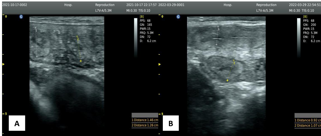
Figure 2. A, An ultrasound image of uterine horns is hyper echoic without a clear lumen due to ovarian inactivity in postpartum anestrous using a 5 MHz trans-rectal transducer. B, An ultrasound image of uterine horns shows gray transparent uterine layers due to ovarian activity in cyclic cows by using 5 MHz trans-rectal transducer.
